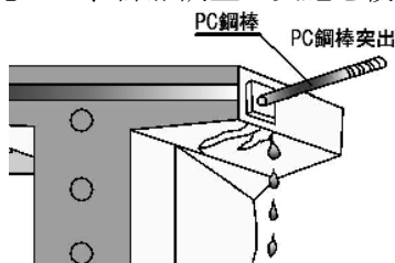
図7-2 PC横締鋼棒の破断
