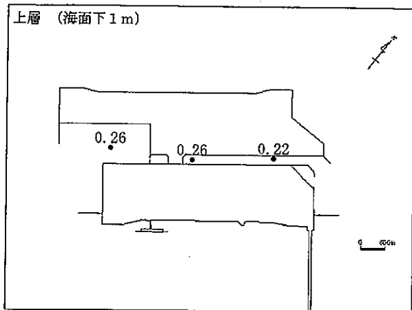
T-N [mg/L]
